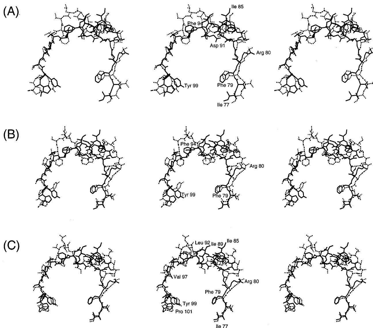
FIGURE 8 Three-dimensional stereo-plots showing the difference between the active site lid (Ile-77–Pro-101) taken from the crystal structure (4tgi) and lid conformations taken along the trajectory from the Rml-product-patch simulations. Solid curve represents the active site lid from the crystal structure, whereas the dash line represents lid configurations at 450 (A), 1130 (B), and 2000 ps (C).
